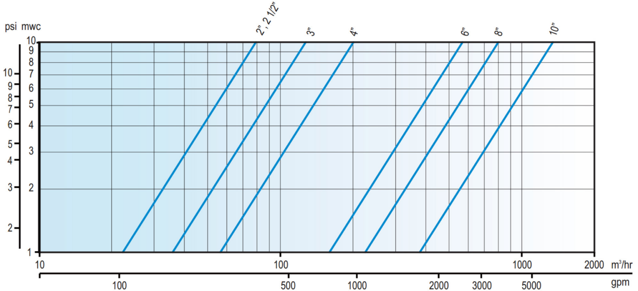
Model SD-DVH-PT680 Head Loss
