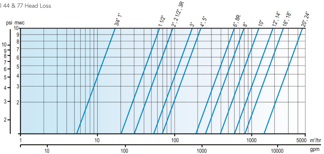
Model 44 & 77 Hydraulic Characteristics (UL Listed diameters shown in chart)
