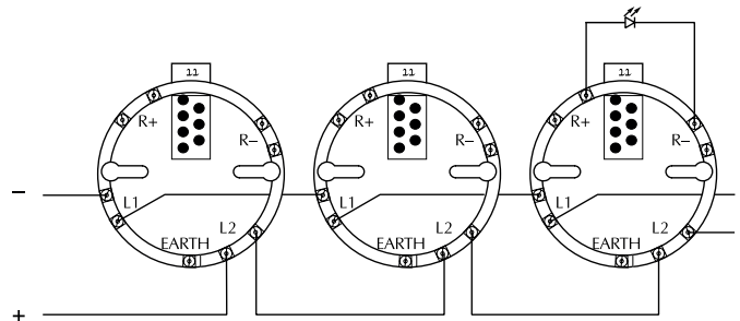
Fig. 2 - Wiring diagram of loop with a common remote LED
