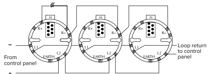
Fig. 2 - Wiring diagram of loop with a common remote LED
