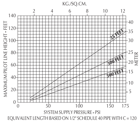
WET PILOT SPRINKLER HEIGHT LIMITATION OF 80NB
