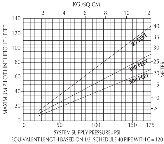
WET PILOT SPRINKLER HEIGHT LIMITATION OF 100NB
